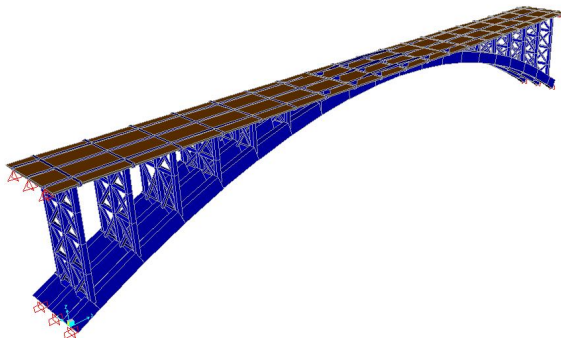
Figure 3: Braced model
