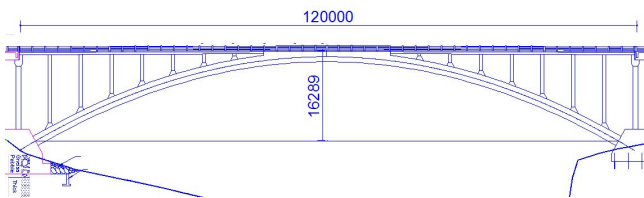
Figure 1: Sectional Elevation of the Bridge
