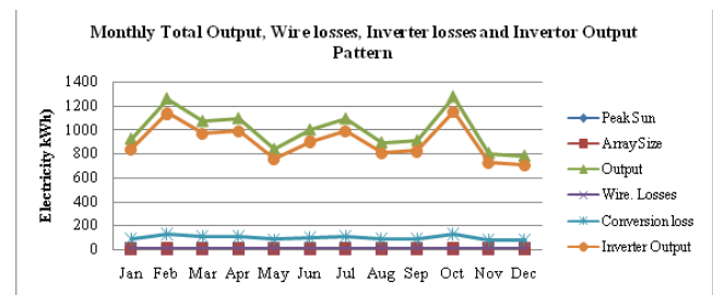
Figure 8: Monthly Energy Output, wire losses, Inverter loss and Inverter output of BIPV
