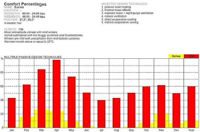
Figure 13: Multiple passive design techniques
